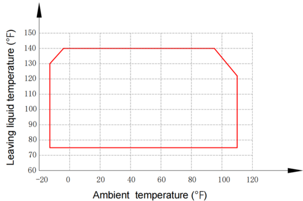
Heating operation envelope
